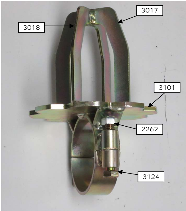
3110-XL Clamp-On Extended Spring Cup
