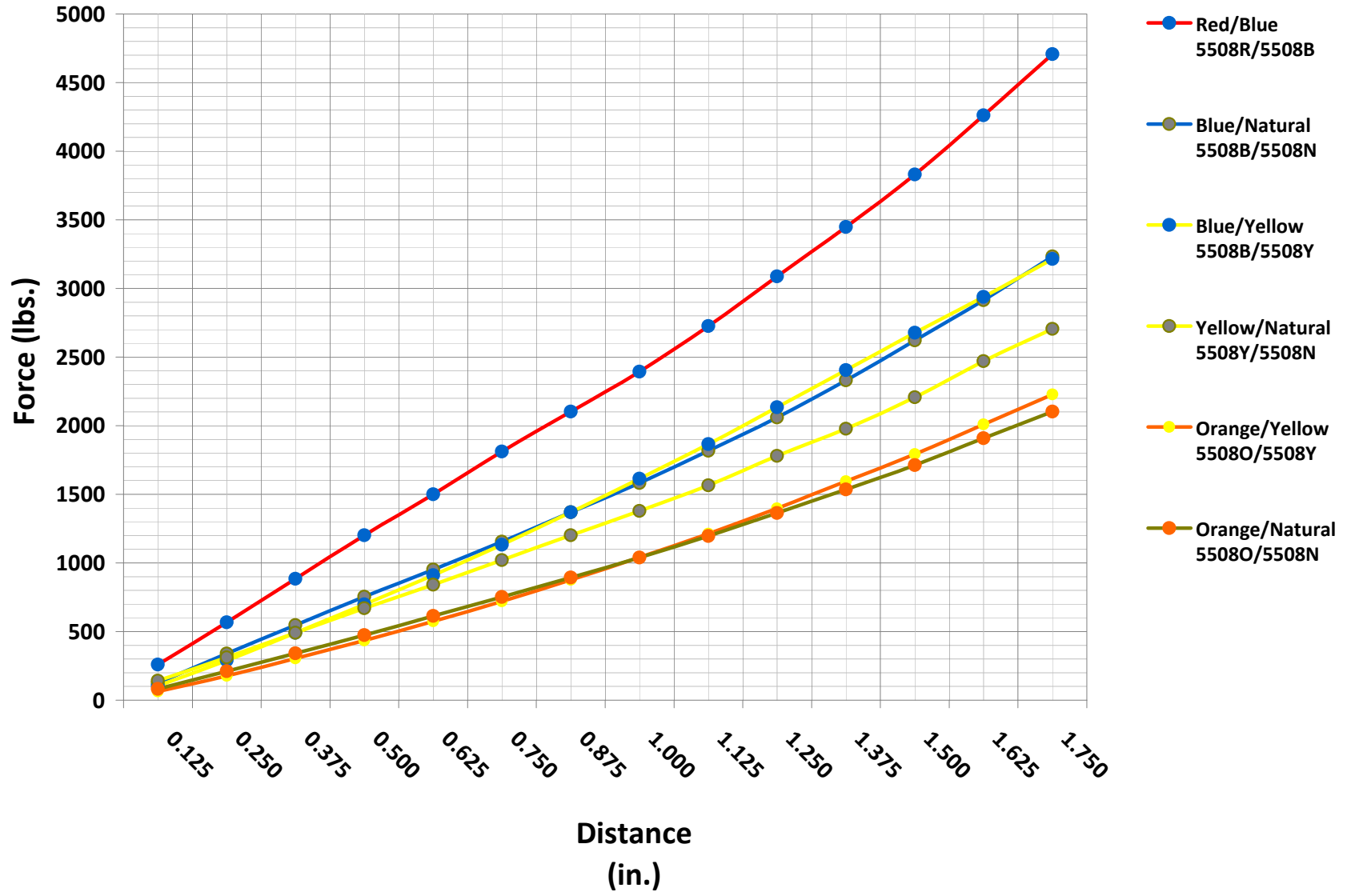
5508 Two Bushing Combination Graph
