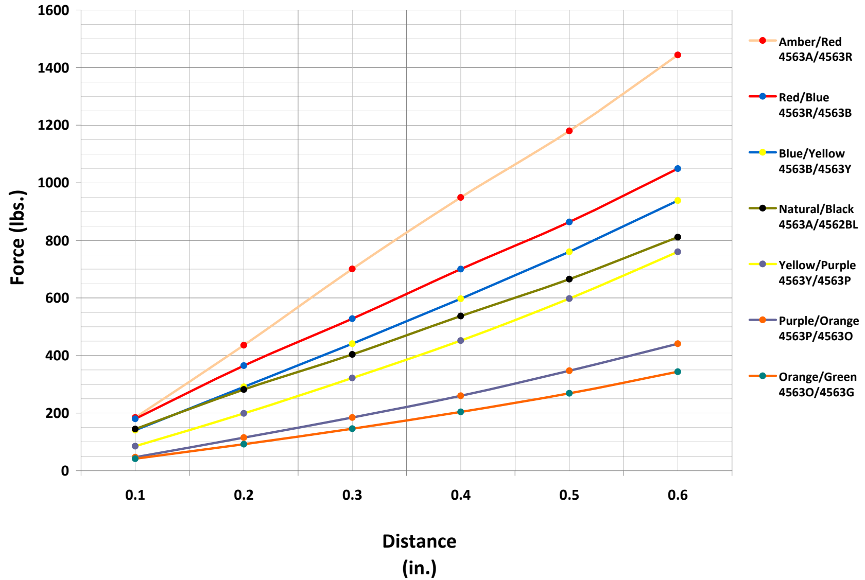
4563 Two Combination Bushing Compression Graph
